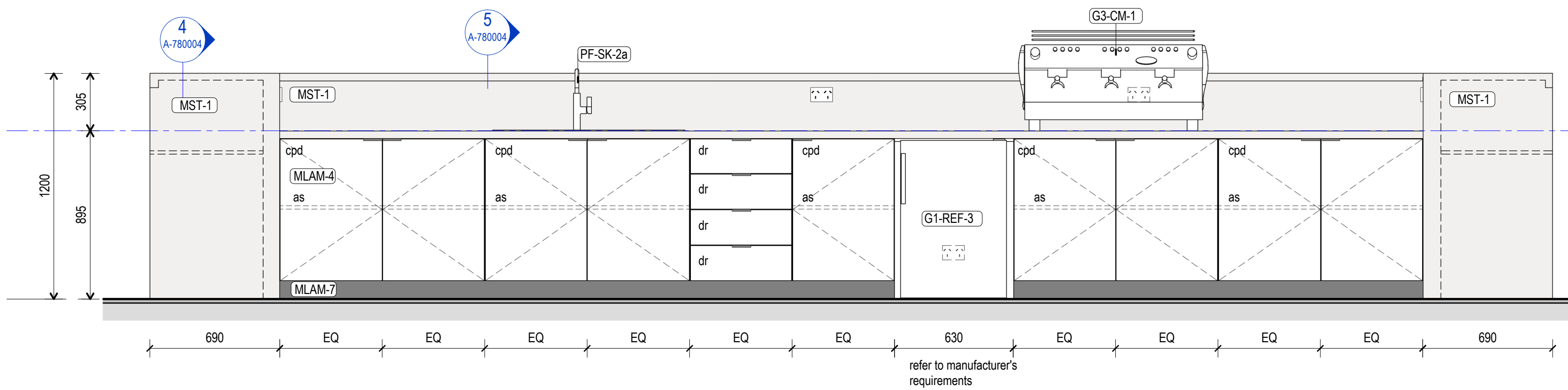
3 JO-BW-1 Elevation 1 : 20
