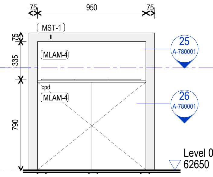
7 JO-BW-1 Elevation 3 1 : 20
